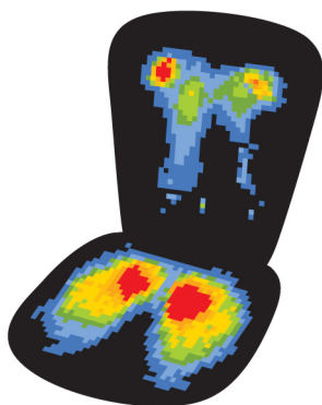
/ Figure 2 / Good pressure distribution in a chair focuses peak pressure under the sitting bones in upright postures and in the lumbar and thoracic areas in reclined postures.
